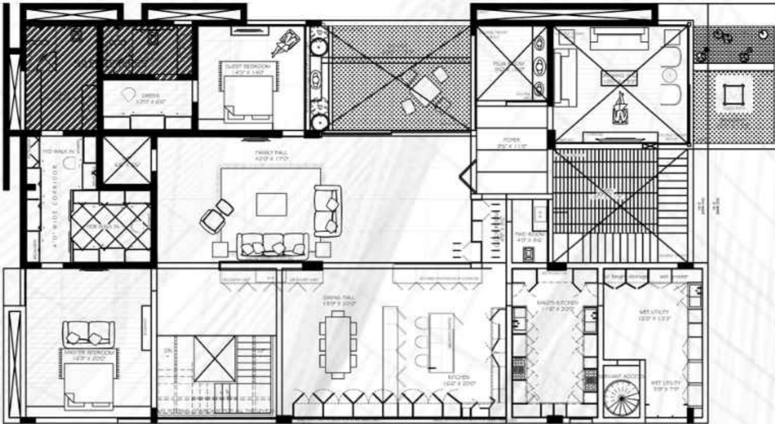
SECOND FLOOR
