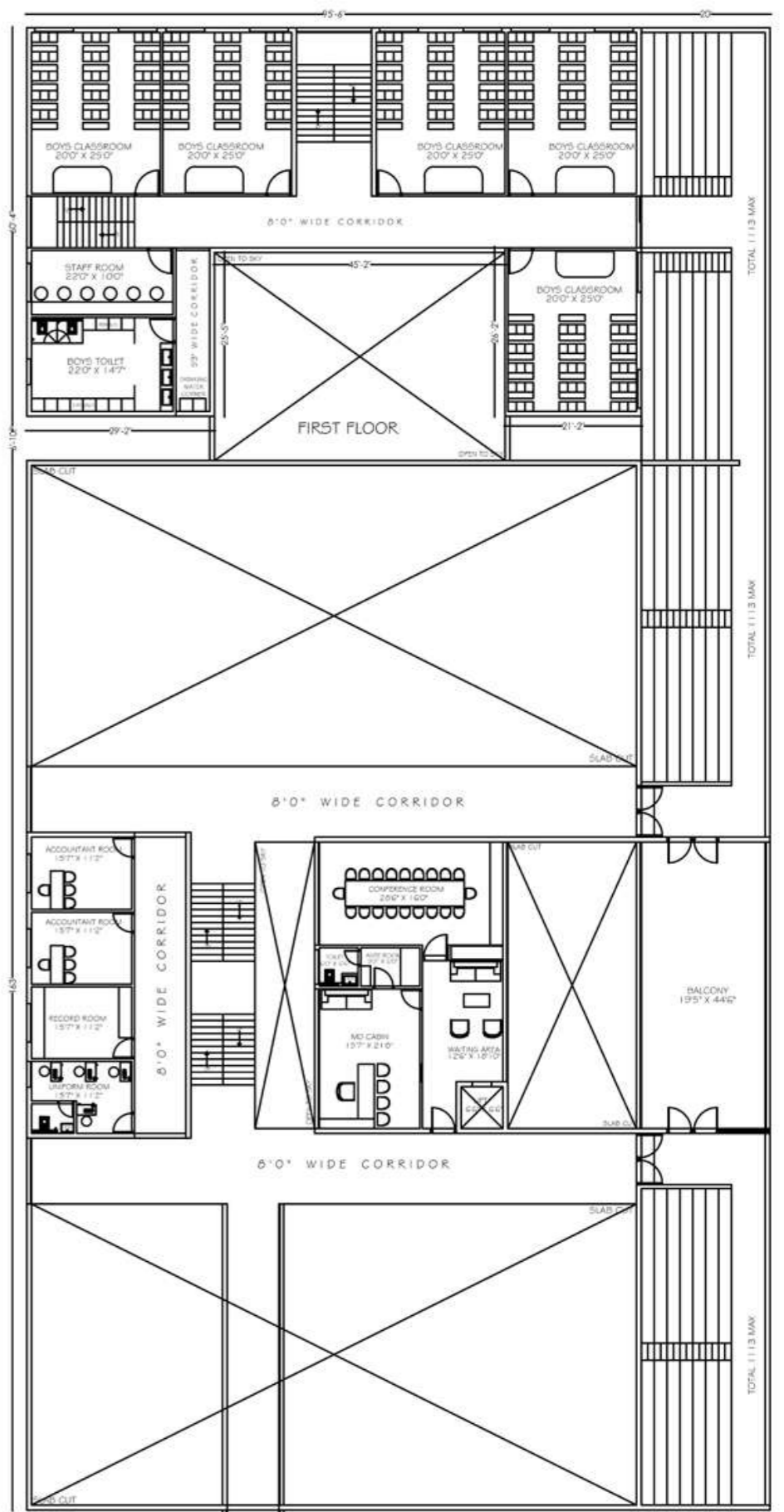
FIRST FLOOR
