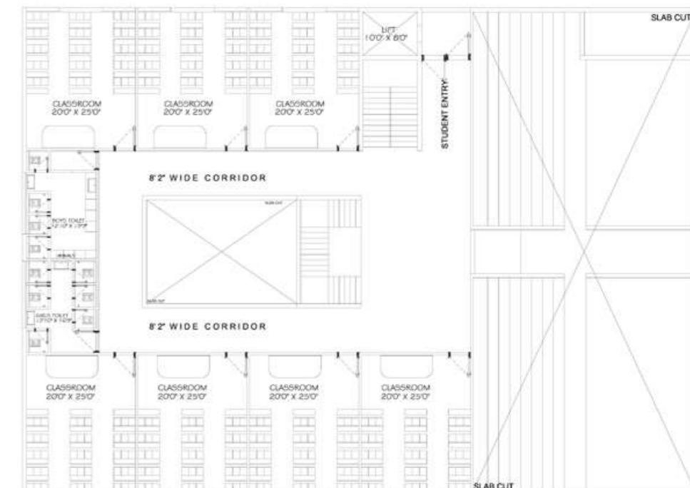
SECOND FLOOR
