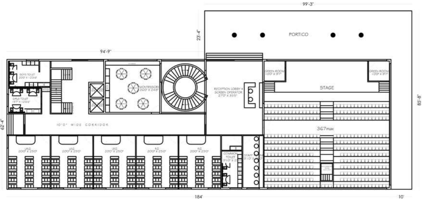
GROUND FLOOR
