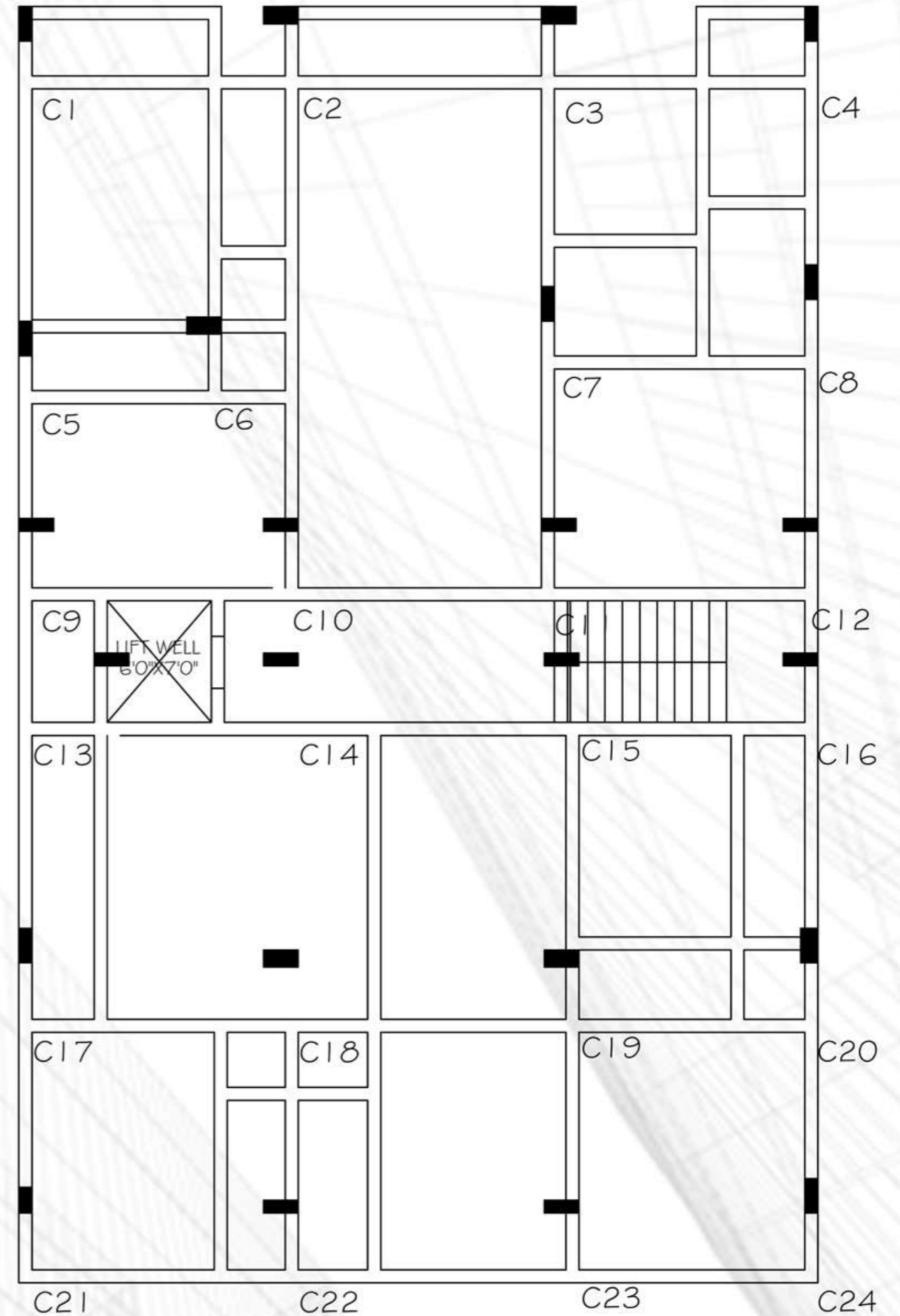
BEAM & COLUMN LAYOUT
