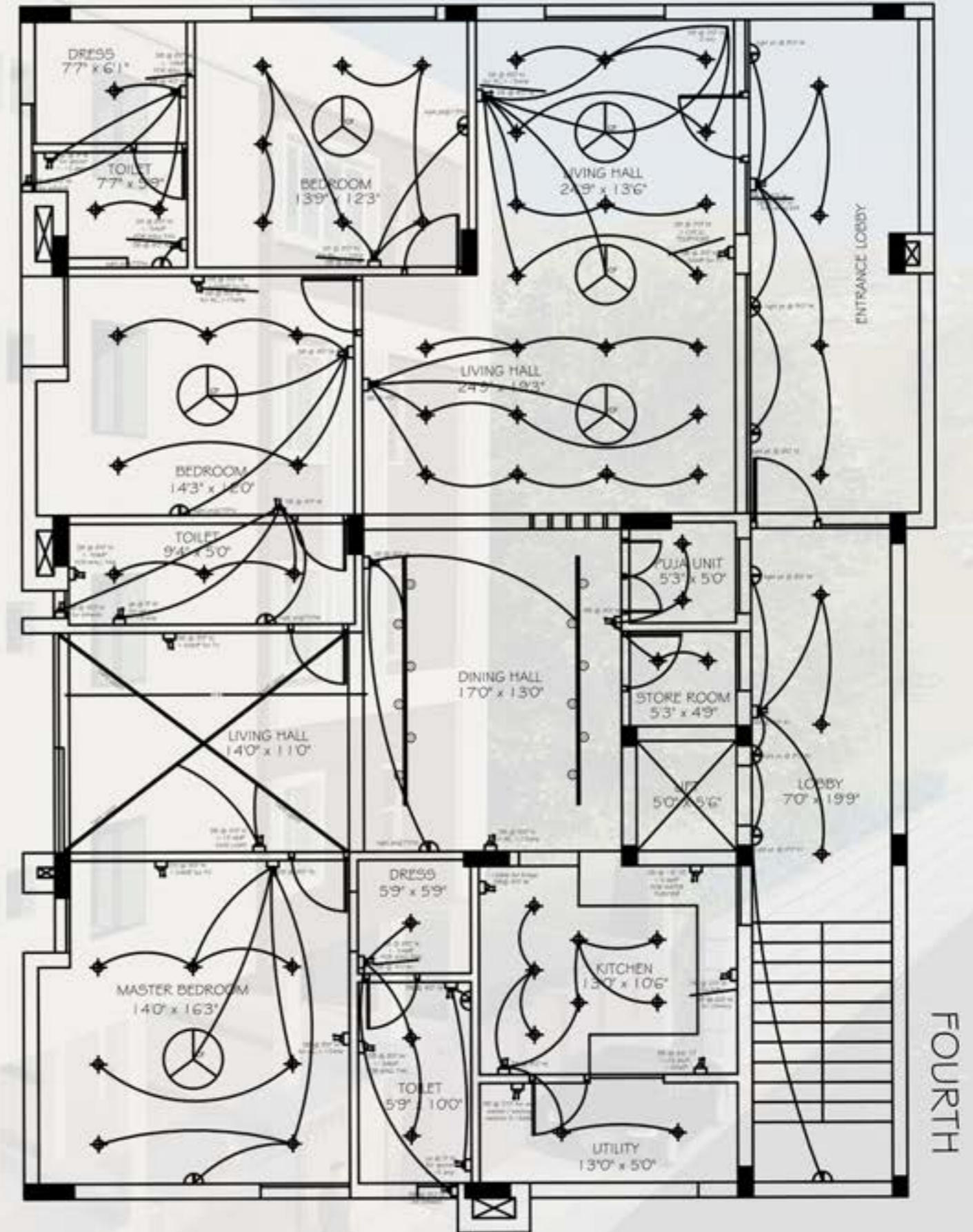
ELECTRICAL DRAWING
