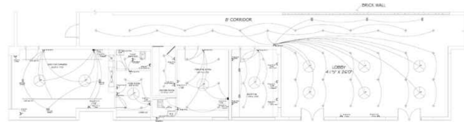
ELECTRICAL PLAN
