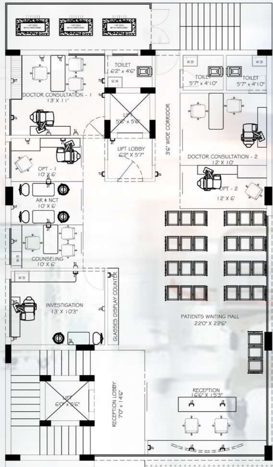
SECOND FLOOR
